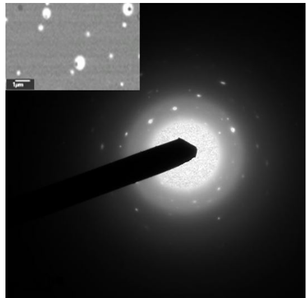
Fig. 4: Electron diffraction pattern indicating crystalline nature of sample; inset SEM image of nanoparticle reach preform core.
